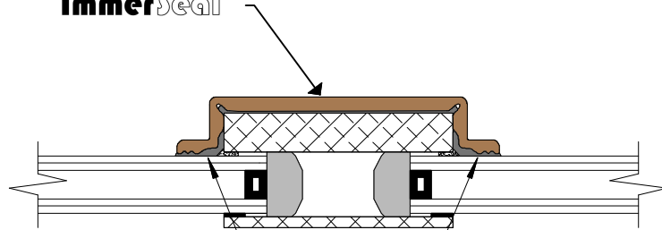
Notches/ Bend-Lines
