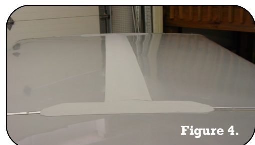
ImmerSeal® installed on the trailer seams
